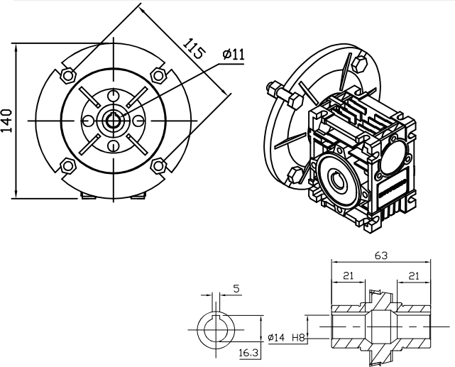
OUTPUT HOLLOW SHAFT
